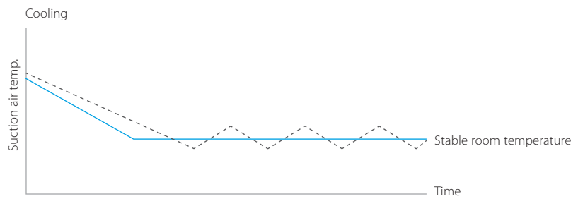
— VRV SERIES (DAIKIN indoor unit (PID controlled)) - - - ON/OFF controlled indoor unit (2.5HP)
